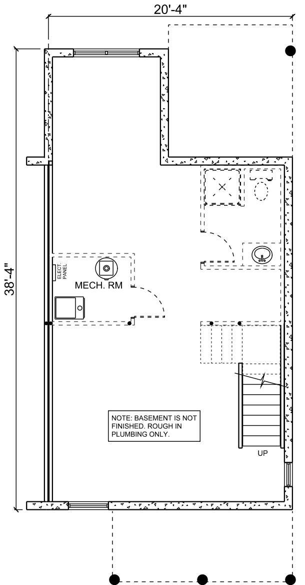
BASEMENT (UNFINISHED): 686 SQ FT
