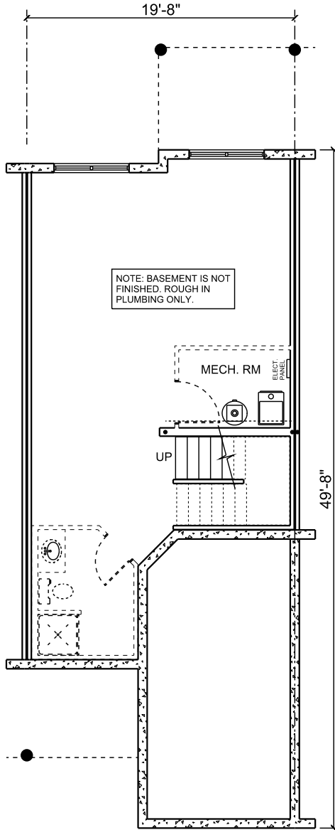
BASEMENT (UNFINISHED): 637 SQ FT
