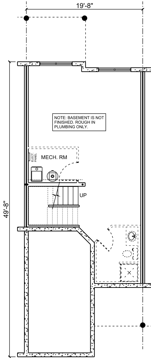
BASEMENT (UNFINISHED): 637 SQ FT
