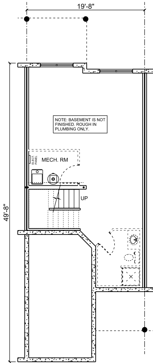
BASEMENT (UNFINISHED): 637 SQ FT
